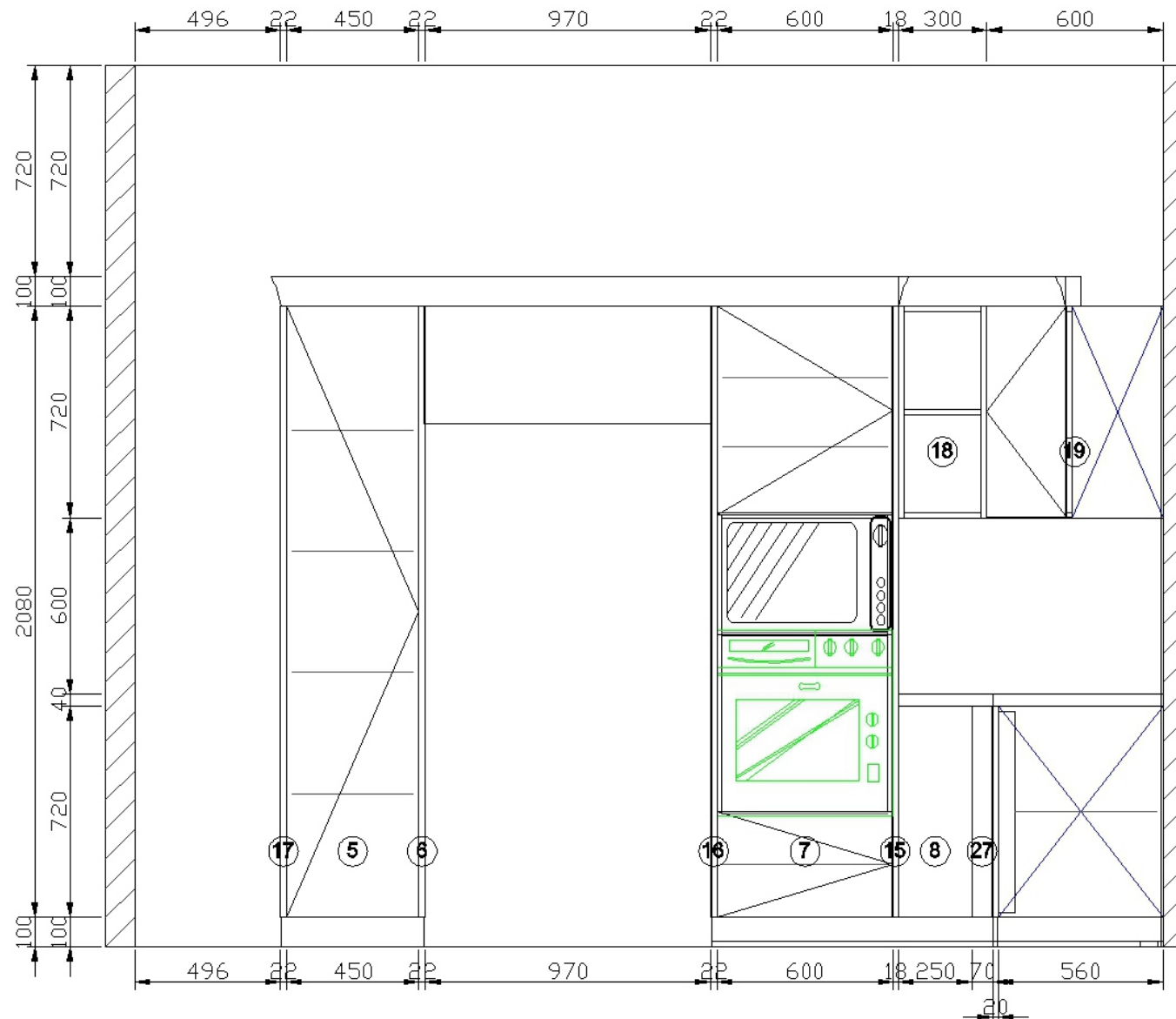
A View elevation drawing
