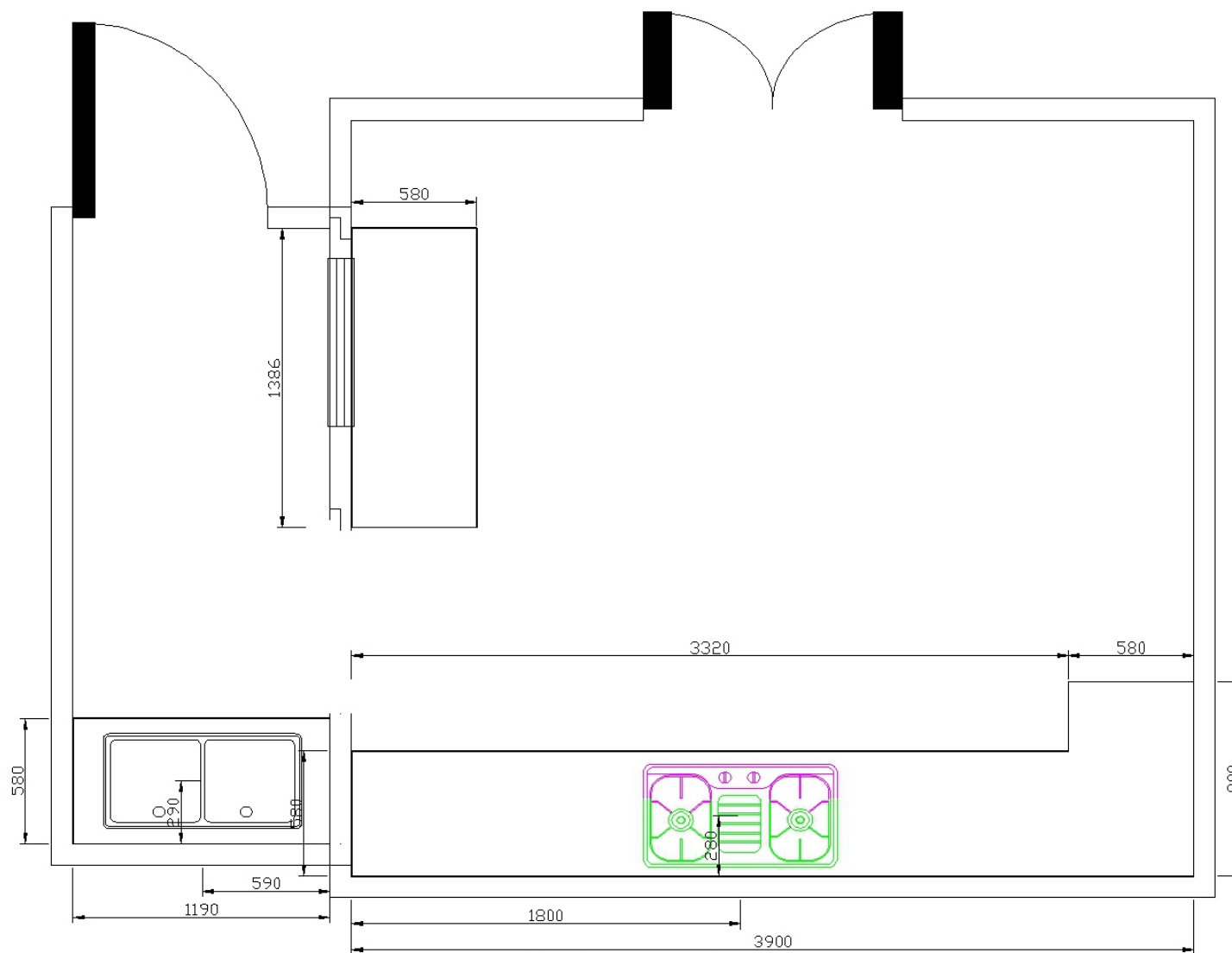
Worktop plan drawing
